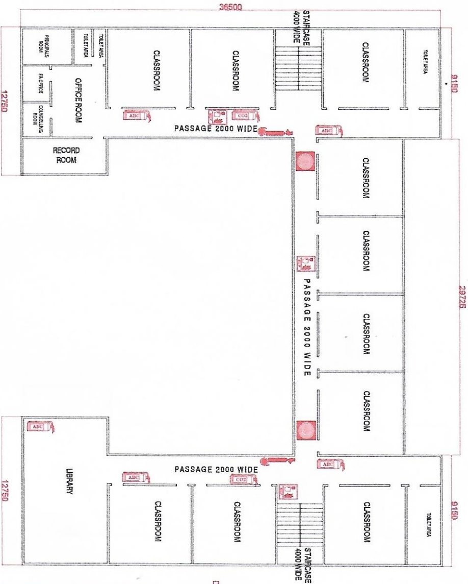
FIRST FLOOR PLAN (USED AS EDUCATIONAL BUILDING)
