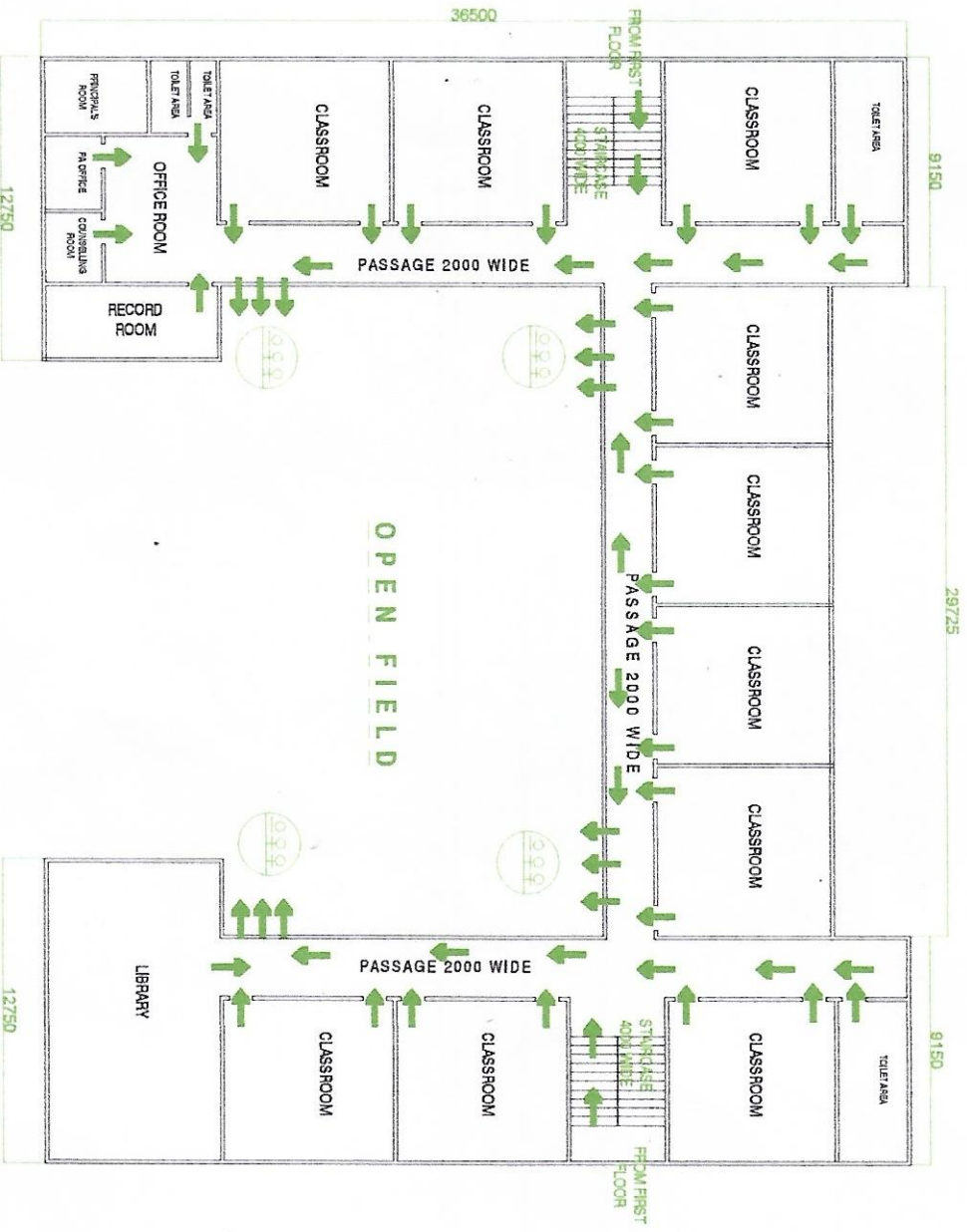
GROUND FLOOR PLAN (USED AS EDUCATIONAL BUILDING)
