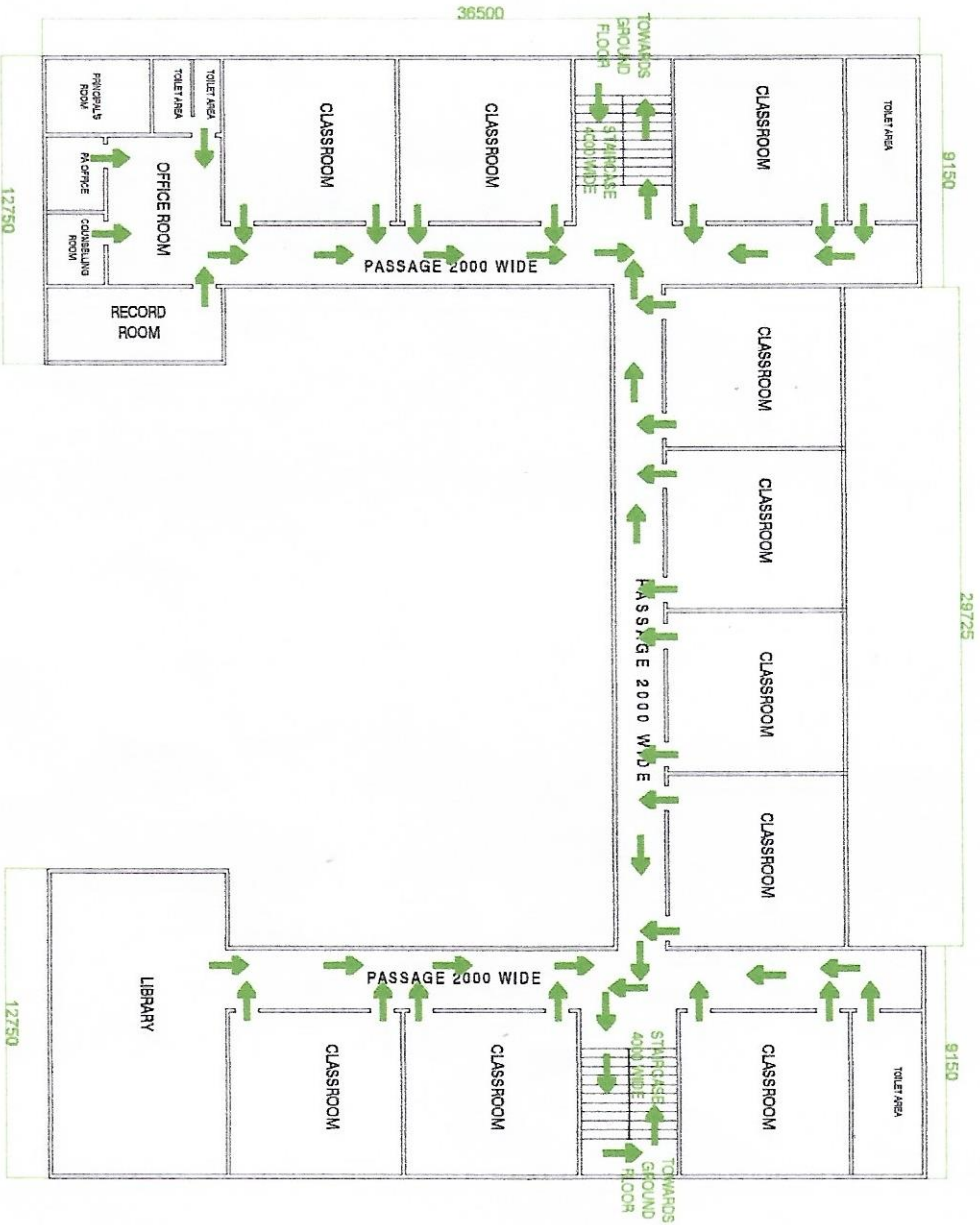
FIRST FLOOR PLAN (USED AS EDUCATIONAL BUILDING)
